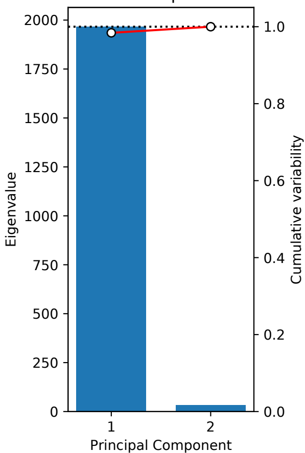
Scree plot
