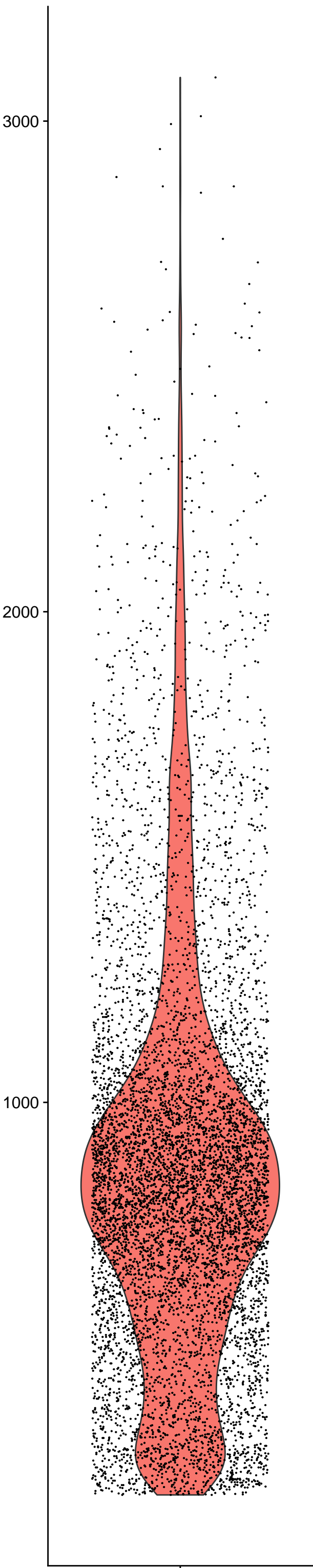
nFeature_RNA
