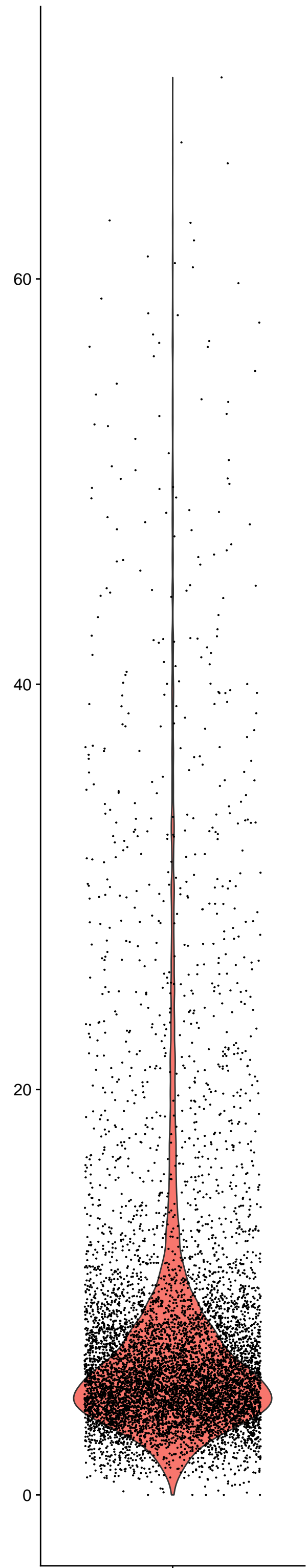
percent.mt
