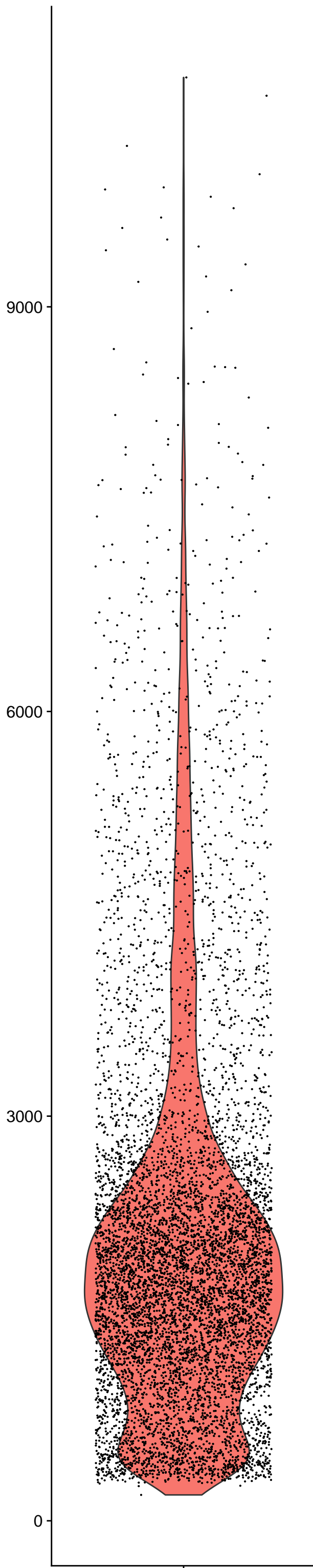
nCount_RNA
