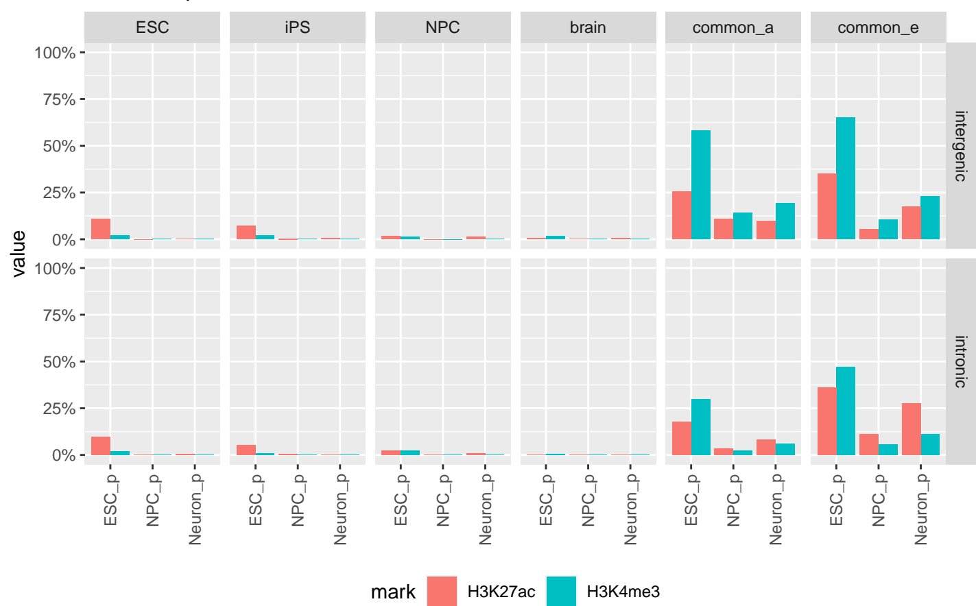
with.input.subsampled_zerone
