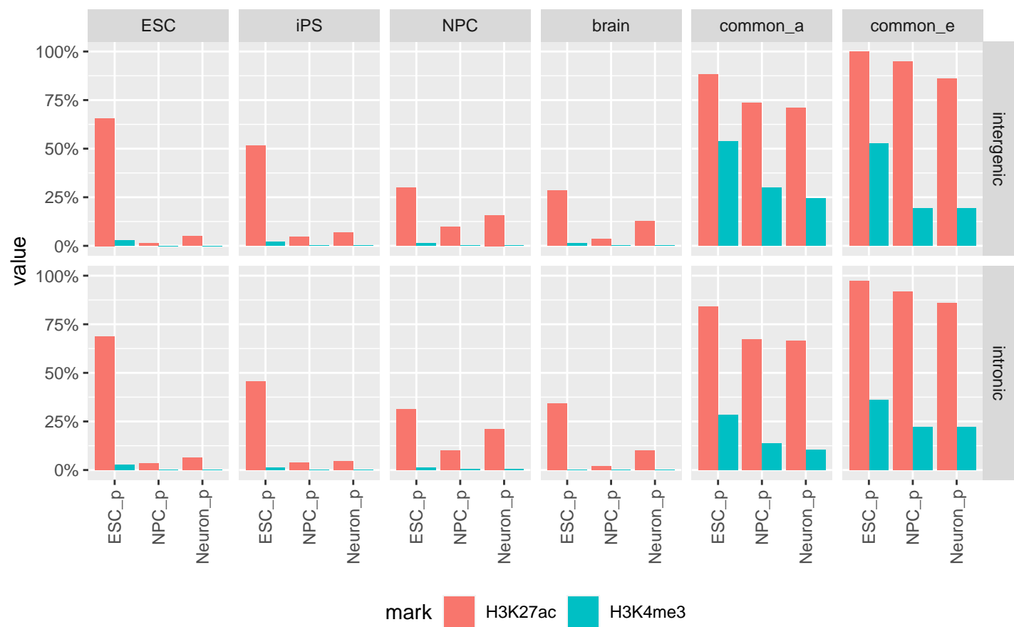
with.input.rep1_zerone
