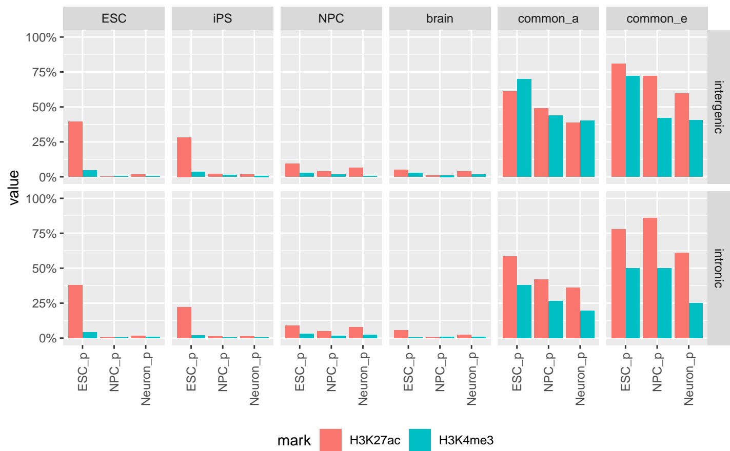
with.input.subsampled.rep1_macs2
