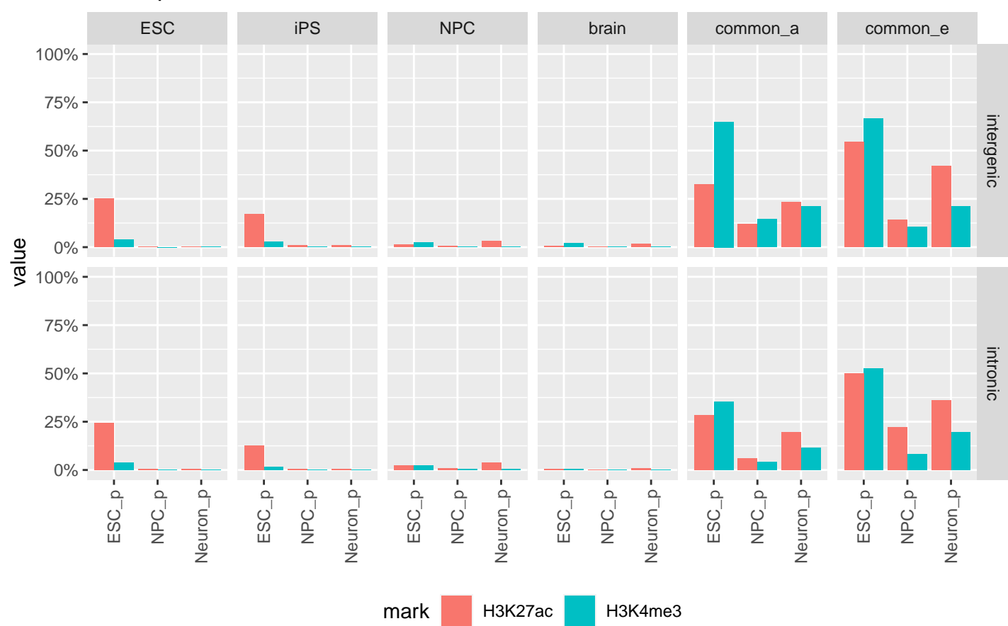
with.input.subsampled_macs2
