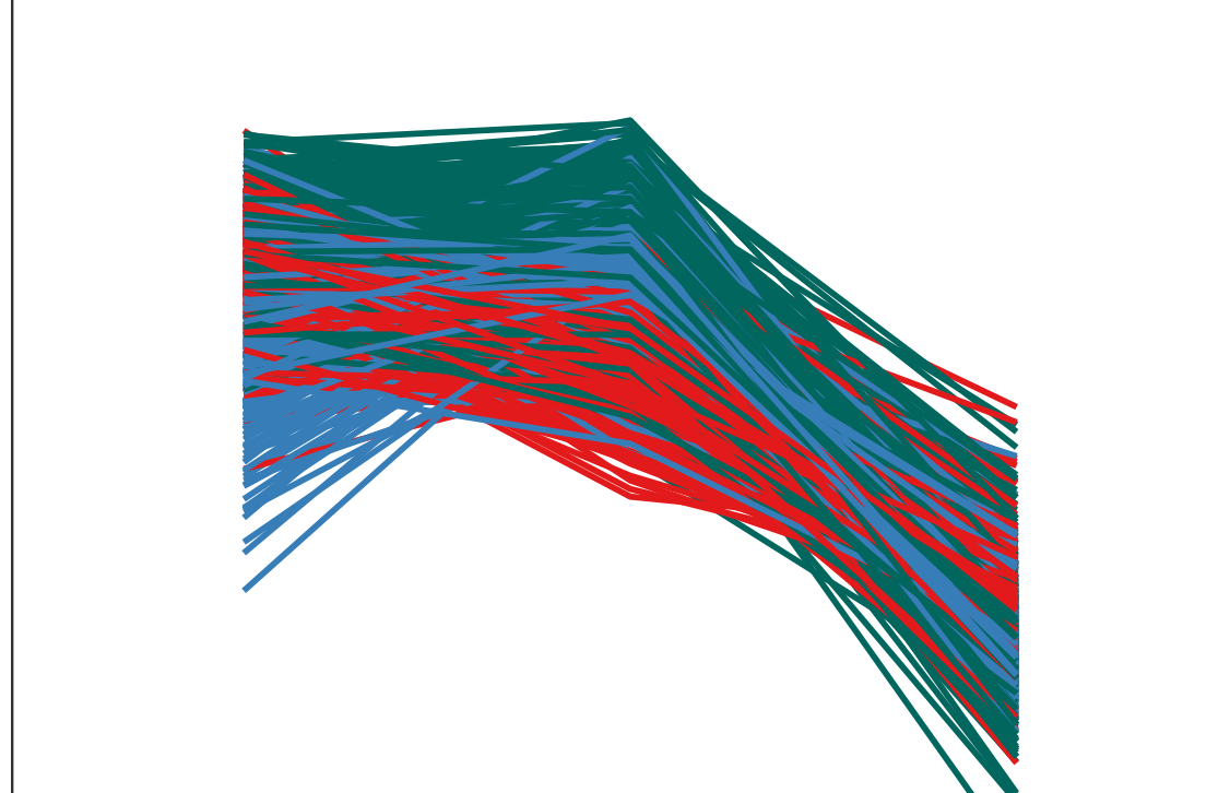
SGs_02_L3_WP_specific
