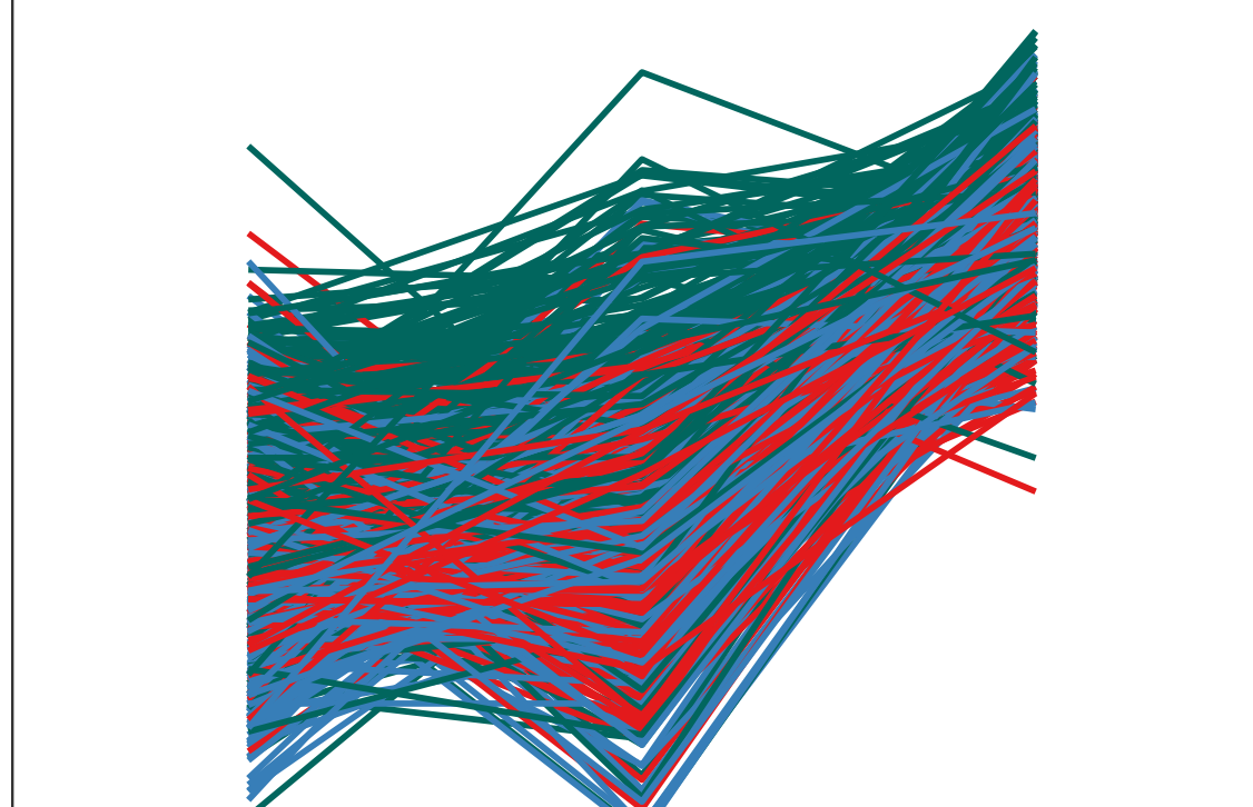
SGs_05_LP_specific
