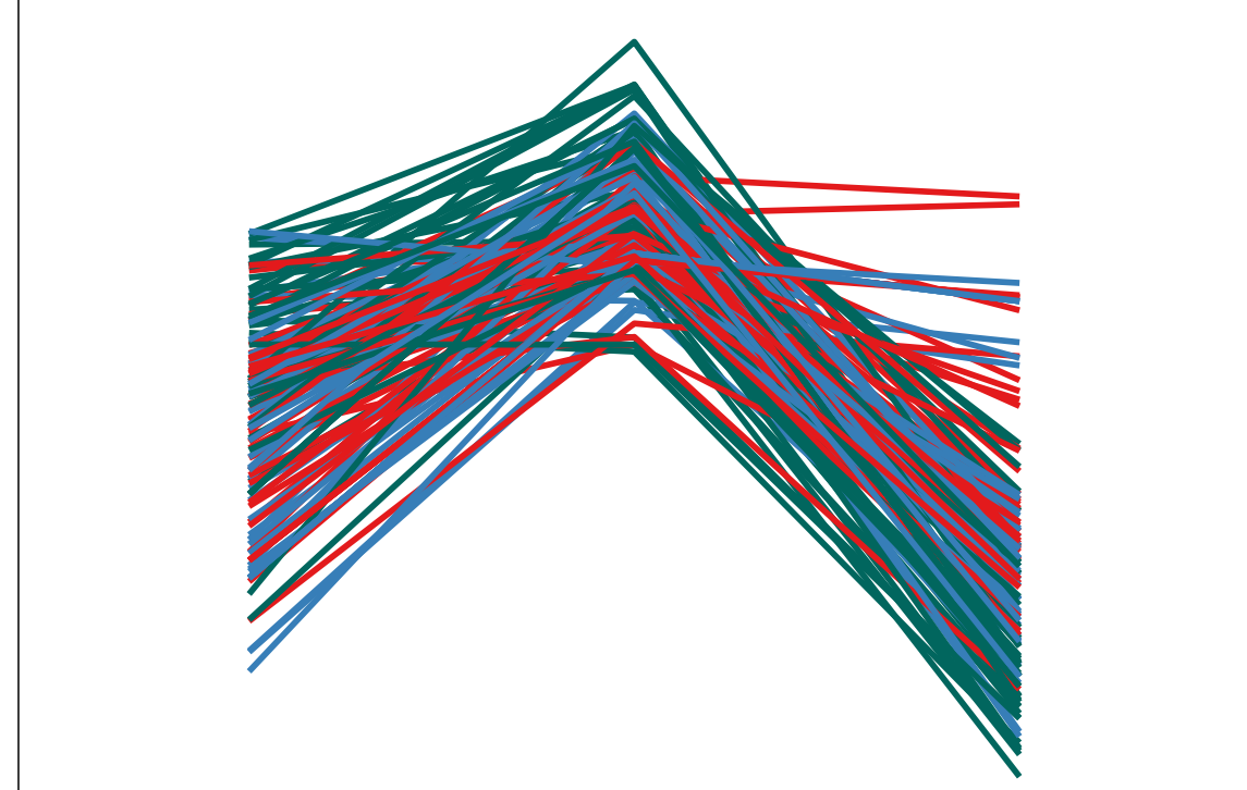
SGs_03_WP_specific
