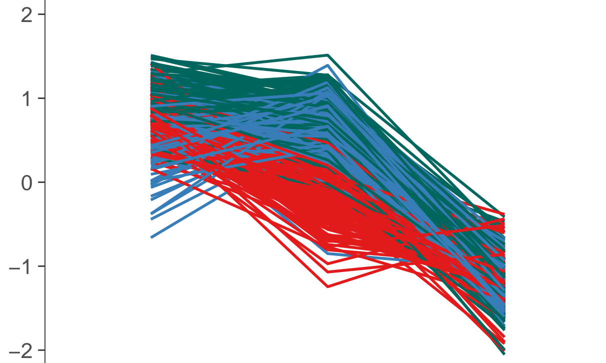
SGs_01_L3_specific
