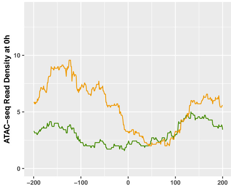
ATAC-seq: genic-intronic (7) upregulated at 0h
