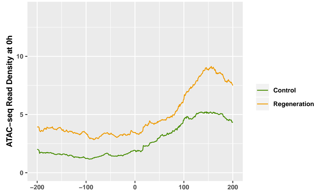
ATAC-seq: genic-exonic (59) upregulated at 0h
