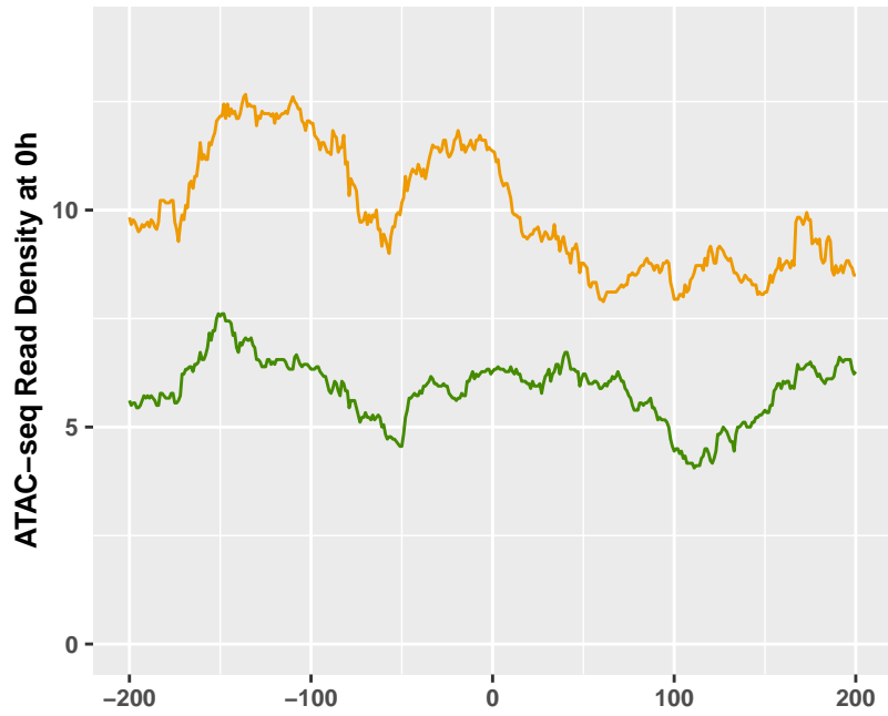
ATAC-seq: lincRNA (18) upregulated at 0h
