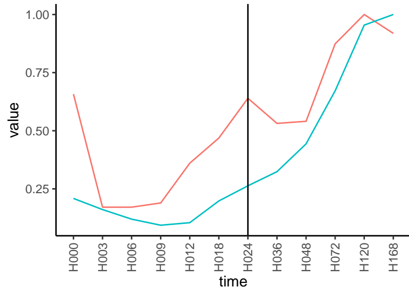
Normalized signals – ENSG00000104043 pre-not-upregulated/post-upregulated
