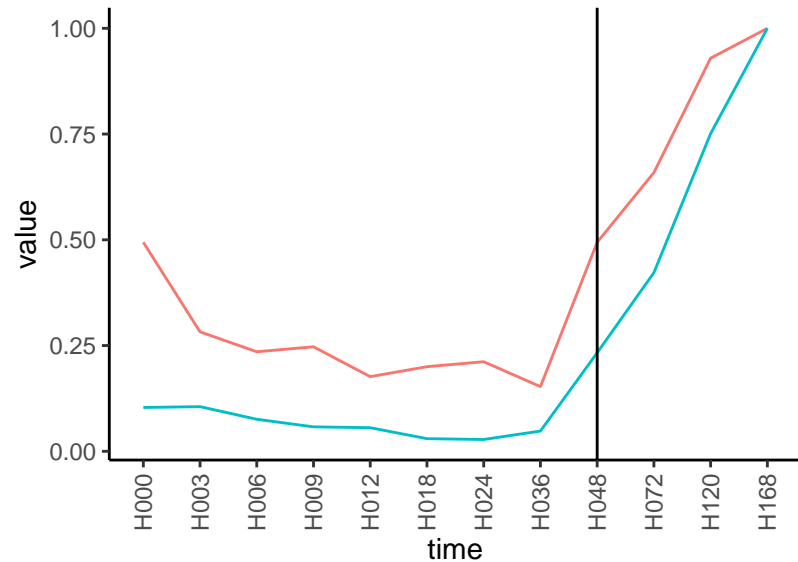
Normalized signals – ENSG00000105697 pre-not-upregulated/post-upregulated
