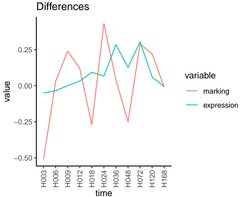
Normalized signals – ENSG00000171777 pre-not-upregulated/post-not-upregulated
