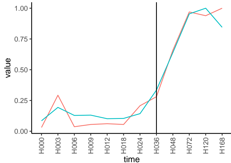
Normalized signals – ENSG00000173166 pre-not-upregulated/post-upregulated
