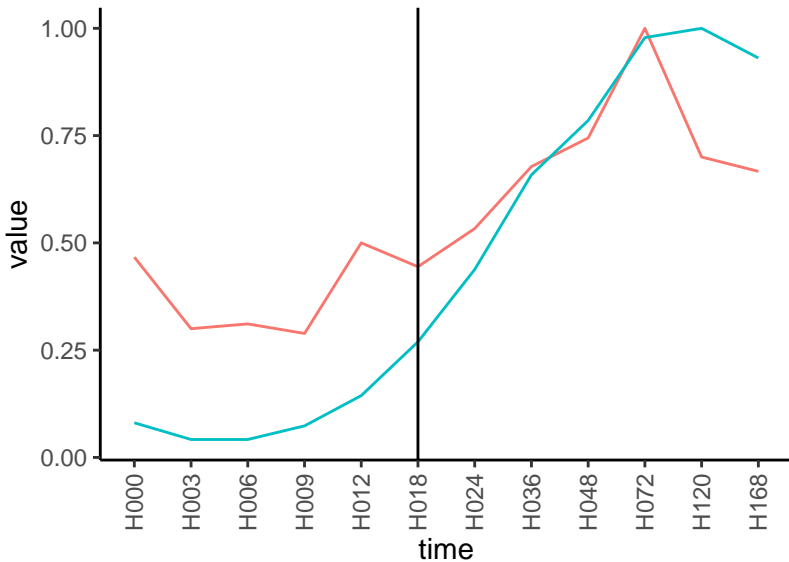
Normalized signals – ENSG00000168329 pre-not-upregulated/post-upregulated
