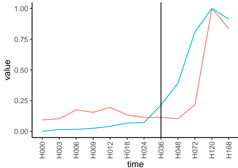
Normalized signals – ENSG00000155659 pre-not-upregulated/post-upregulated
