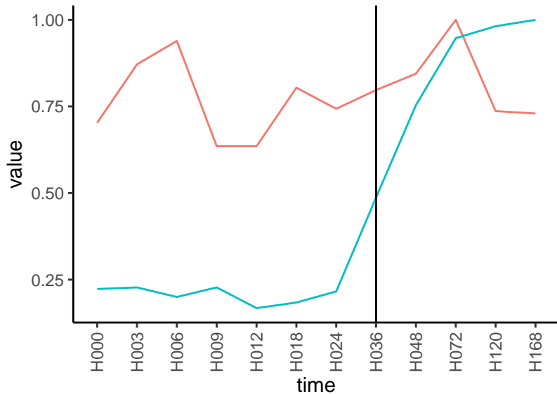
Normalized signals – ENSG00000138640 pre-not-upregulated/post-not-upregulated
