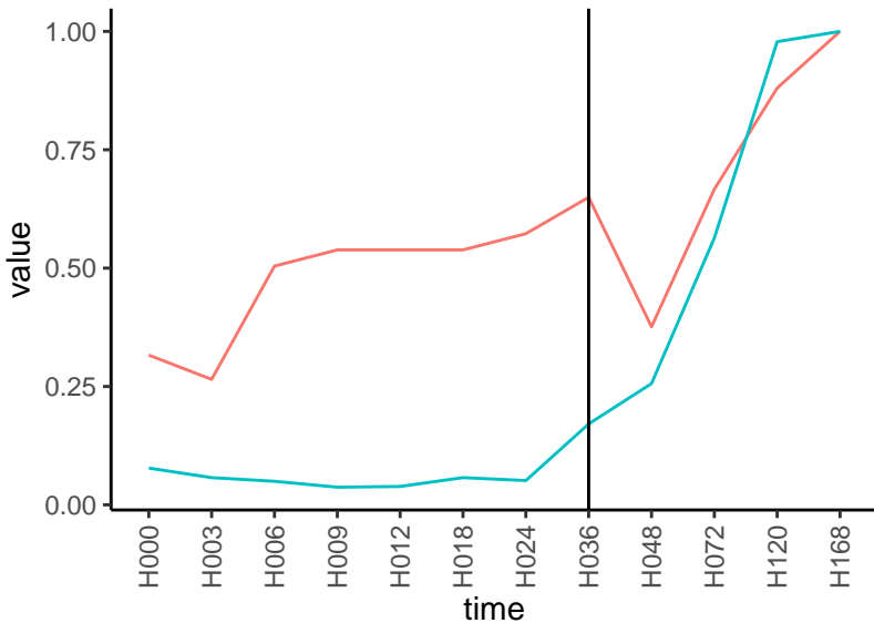
Normalized signals – ENSG00000104921 pre-not-upregulated/post-upregulated
