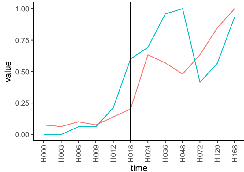
Normalized signals – ENSG00000105352 pre-not-upregulated/post-upregulated
