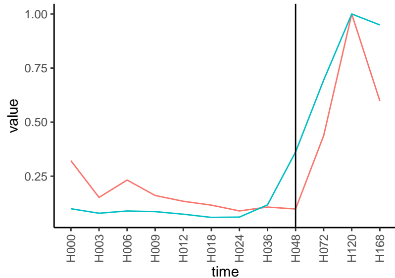
Normalized signals – ENSG00000275395 pre-not-upregulated/post-upregulated
