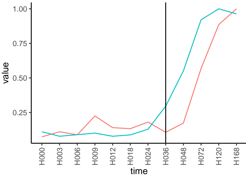
Normalized signals – ENSG00000169403 pre-not-upregulated/post-upregulated
