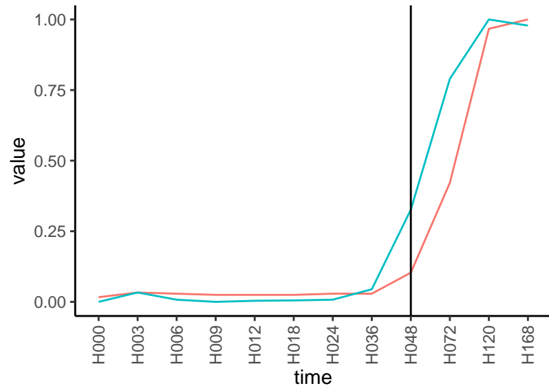
Normalized signals – ENSG00000138135 pre-not-upregulated/post-upregulated
