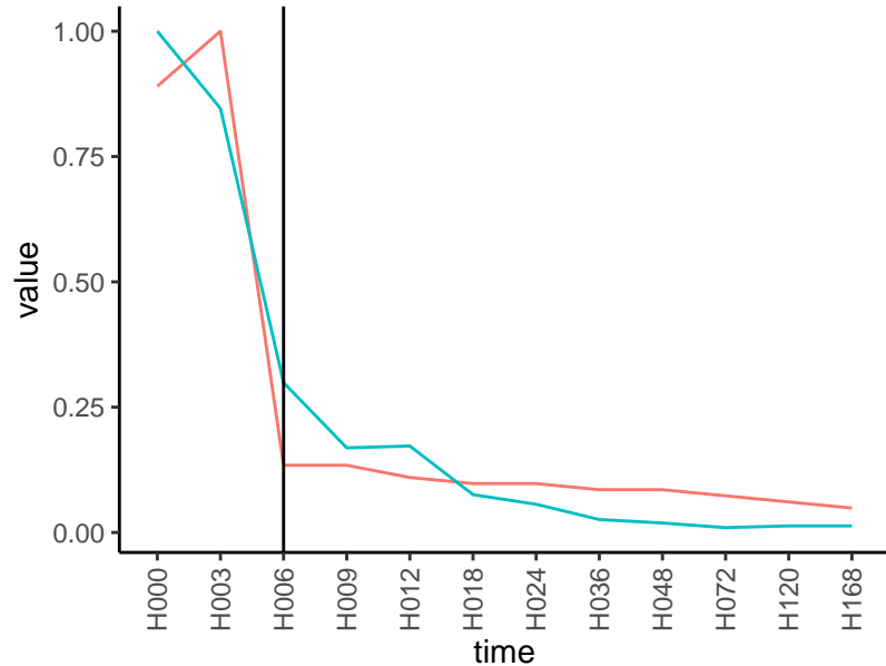
Normalized signals – ENSG00000100290
