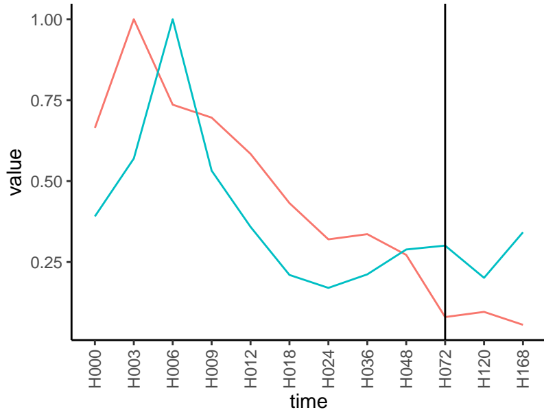
Normalized signals – ENSG00000158292
