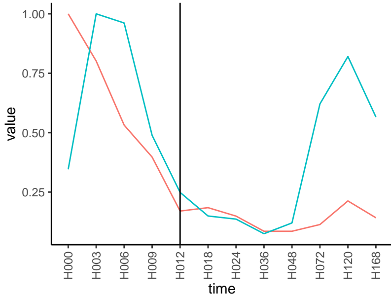
Normalized signals – ENSG00000106089
