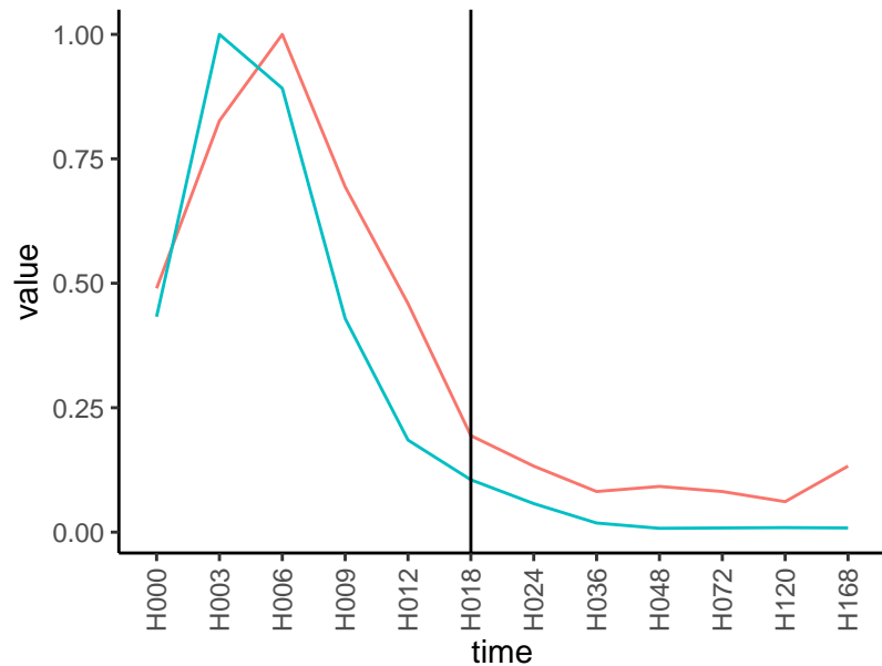
Normalized signals – ENSG00000120278
