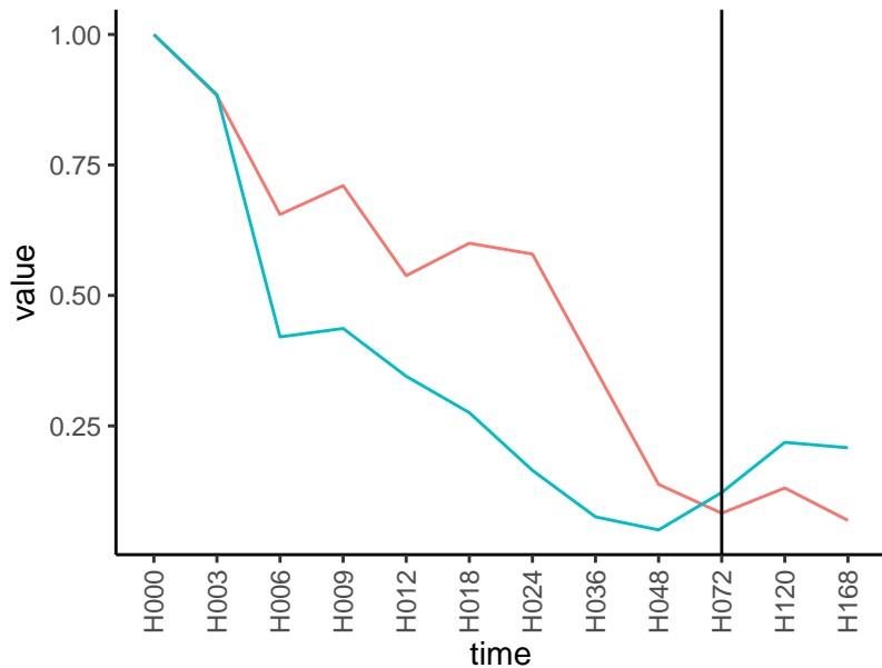
Normalized signals – ENSG00000117016
