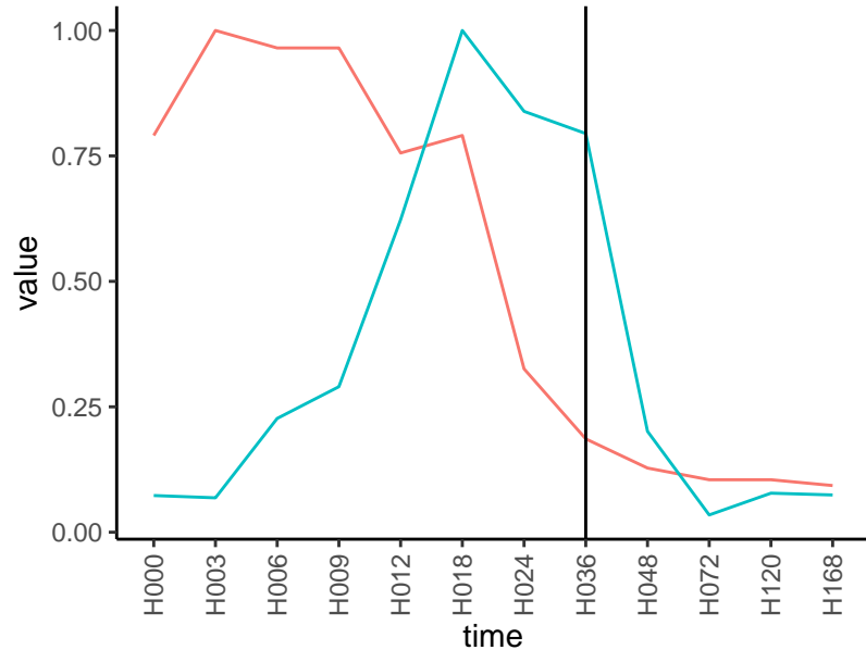
Normalized signals – ENSG00000086548
