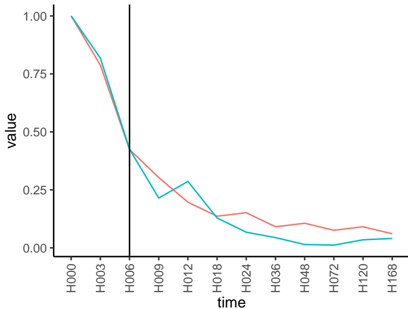
Normalized signals – ENSG00000145506
