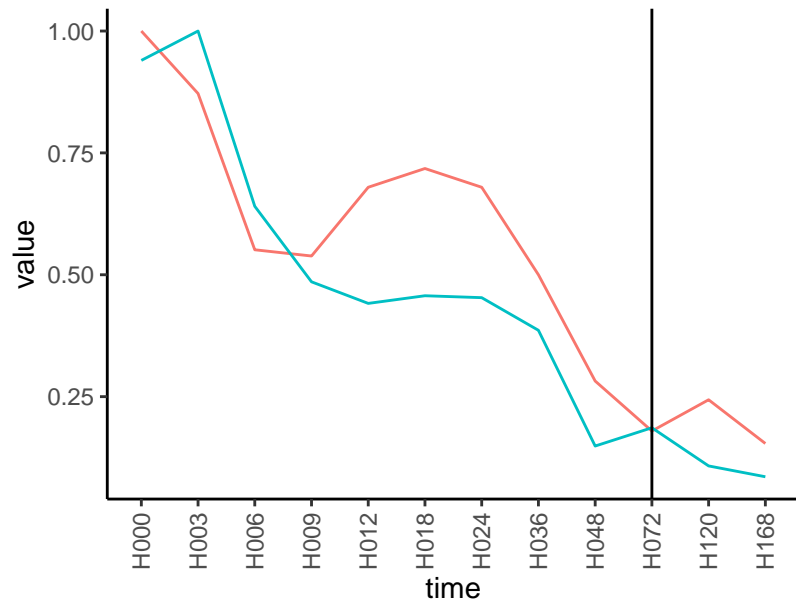
Normalized signals – ENSG00000183018
