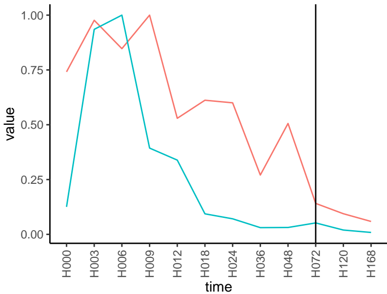
Normalized signals – ENSG00000187479
