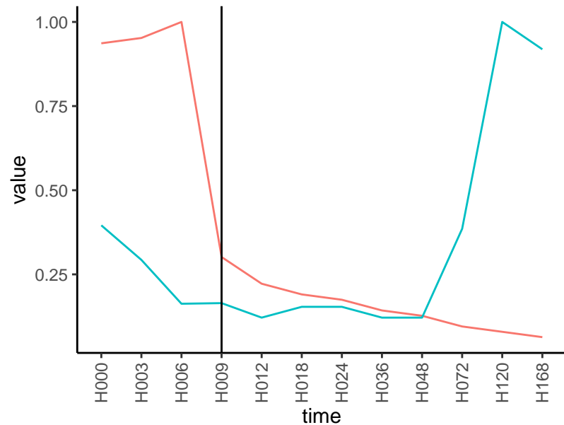
Normalized signals – ENSG00000172824
