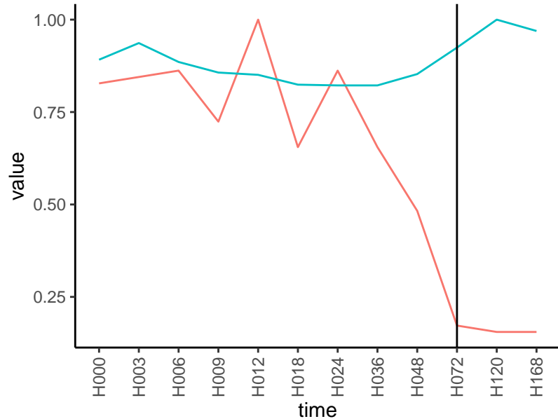
Normalized signals – ENSG00000155313
