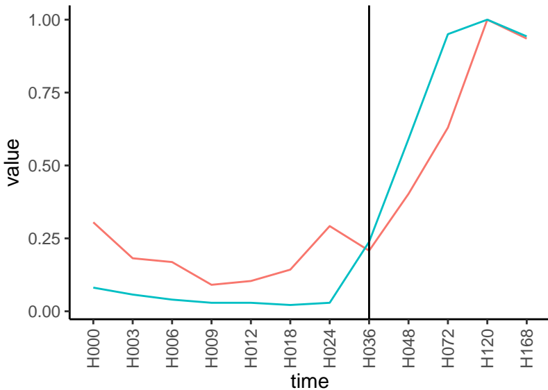
Normalized signals – ENSG00000038945 pre-not-upregulated/post-not-upregulated
