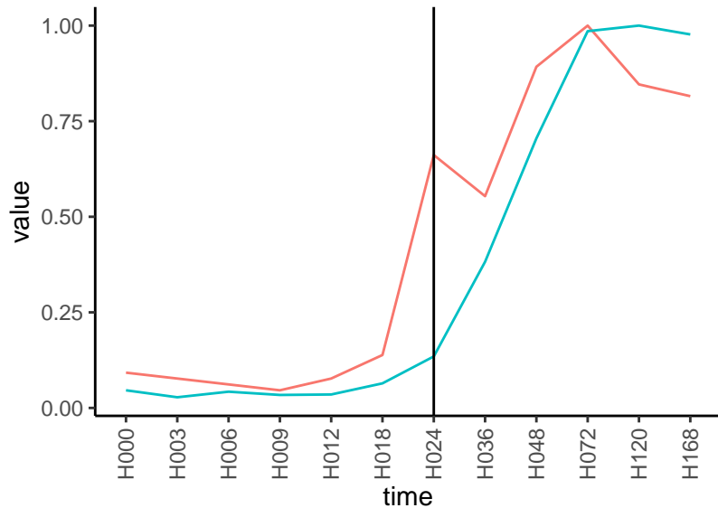
Normalized signals – ENSG00000135218 pre-not-upregulated/post-not-upregulated
