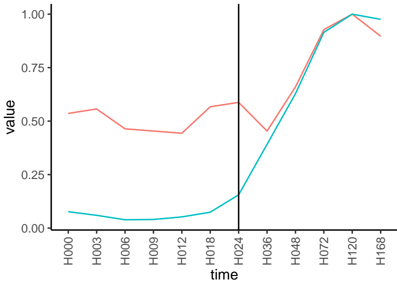
Normalized signals – ENSG00000171860 pre-not-upregulated/post-not-upregulated
