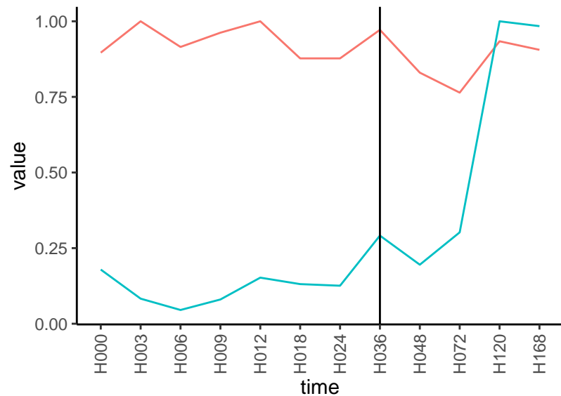
Normalized signals – ENSG00000251380 pre-not-upregulated/post-not-upregulated
