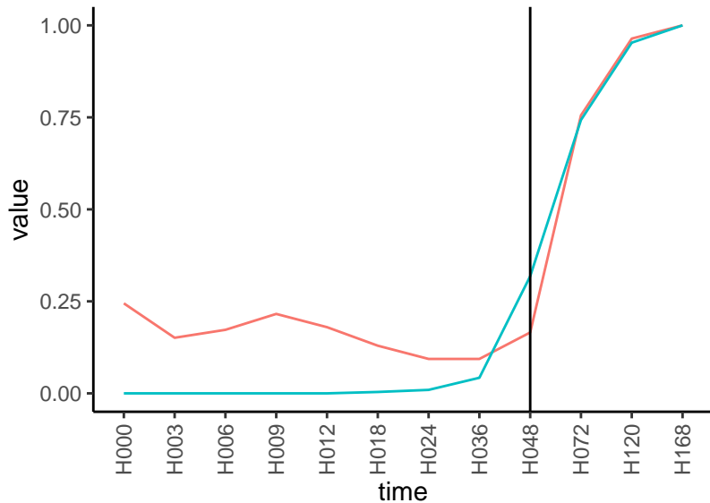
Normalized signals – ENSG00000159189 pre-not-upregulated/post-not-upregulated
