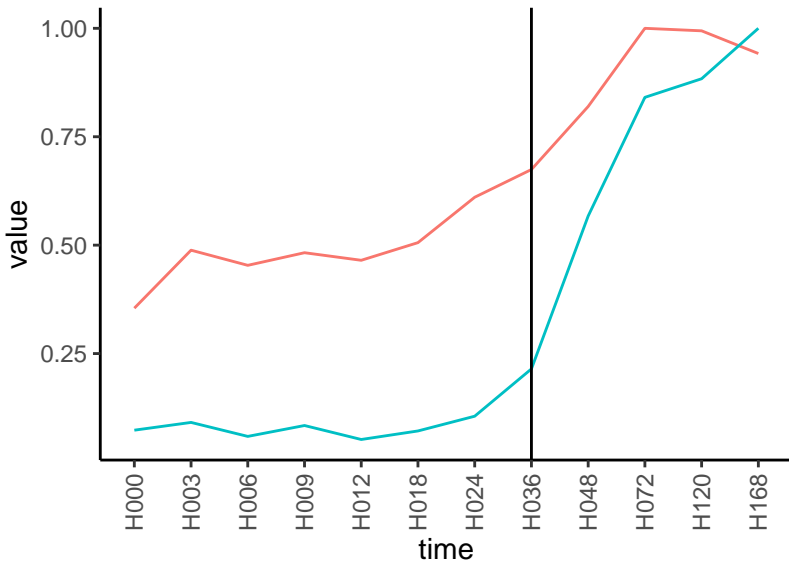
Normalized signals – ENSG00000136634 pre-not-upregulated/post-not-upregulated
