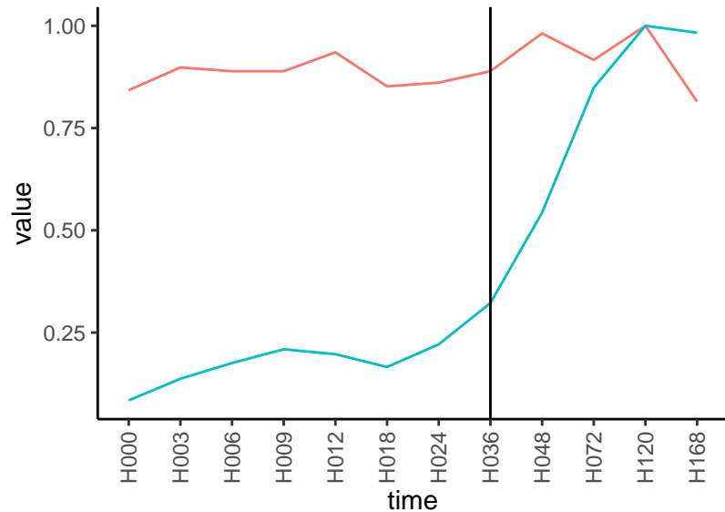
Normalized signals – ENSG00000079215 pre-not-upregulated/post-not-upregulated
