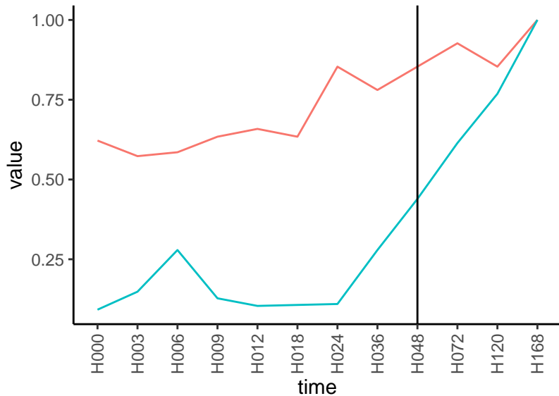
Normalized signals – ENSG00000137726 pre-not-upregulated/post-not-upregulated
