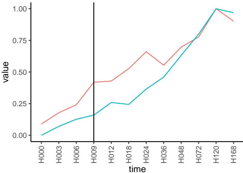
Normalized signals – ENSG00000166523 pre-not-upregulated/post-not-upregulated
