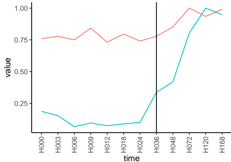
Normalized signals – ENSG00000133106 pre-not-upregulated/post-upregulated
