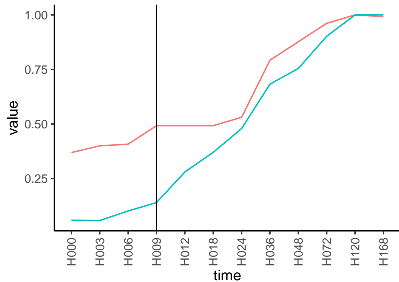
Normalized signals – ENSG00000163823 pre-not-upregulated/post-upregulated
