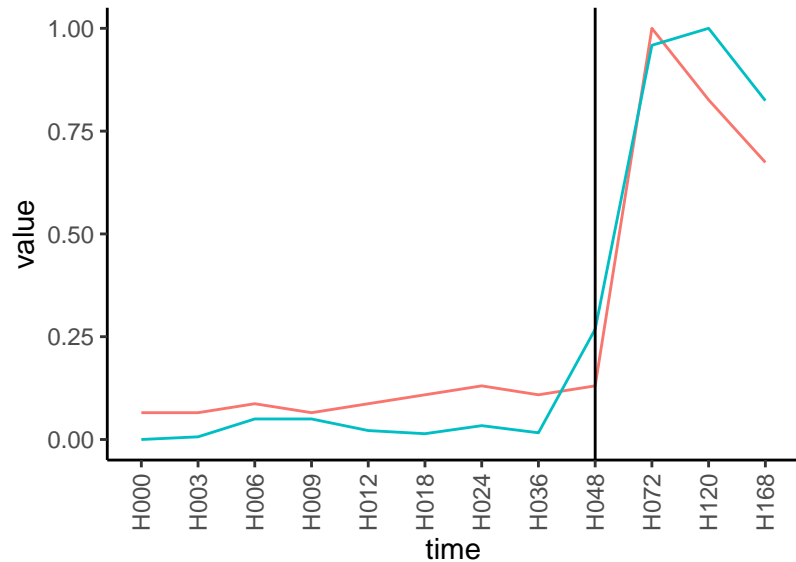
Normalized signals – ENSG00000196611 pre-not-upregulated/post-not-upregulated
