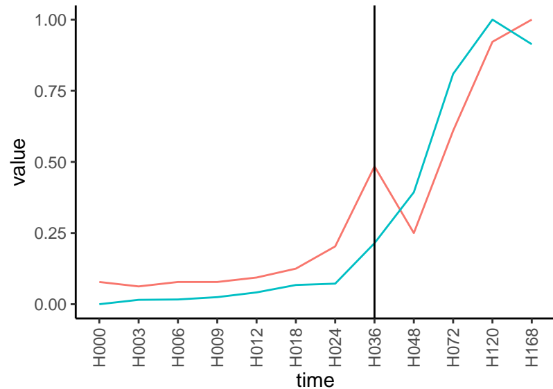
Normalized signals – ENSG00000155659 pre-not-upregulated/post-upregulated
