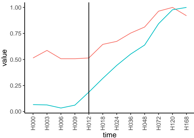
Normalized signals – ENSG00000011600 pre-not-upregulated/post-upregulated
