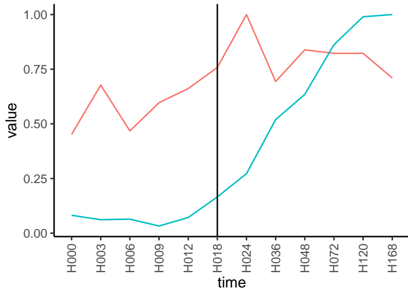
Normalized signals – ENSG00000081237 pre-not-upregulated/post-not-upregulated
