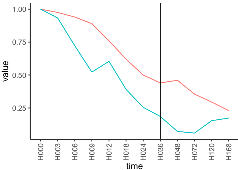
Normalized signals – ENSG00000145506 pre-not-downregulated/post-downregulated
