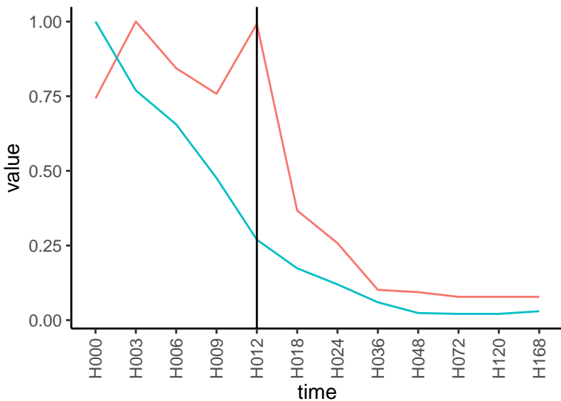
Normalized signals – ENSG00000153822 pre-not-downregulated/post-downregulated
