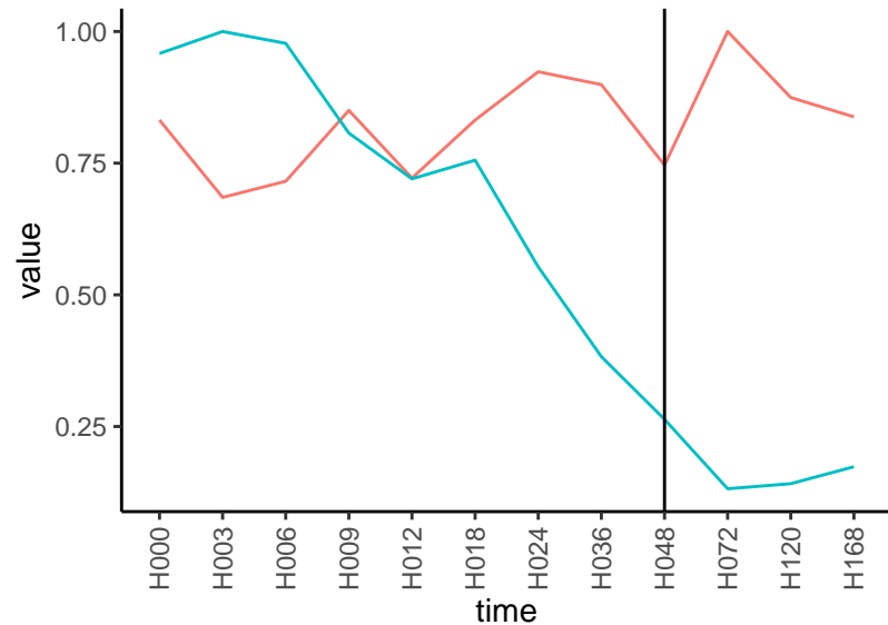
Normalized signals – ENSG00000151376 pre-not-downregulated/post-downregulated
