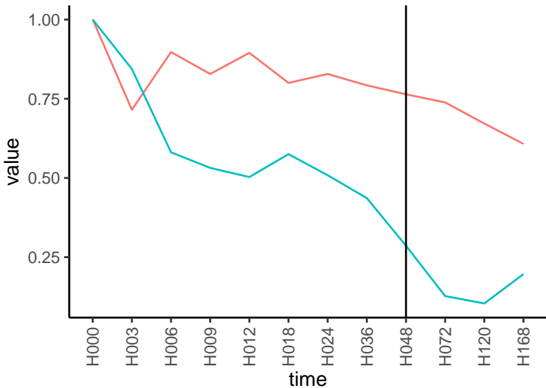
Normalized signals – ENSG00000151692 pre-not-downregulated/post-not-downregula
