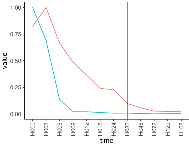
Normalized signals – ENSG00000128322
