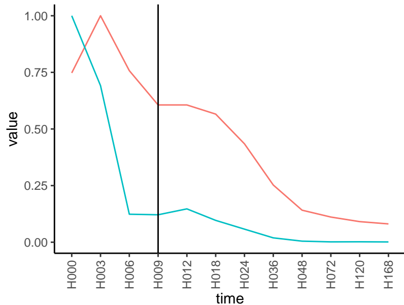
Normalized signals – ENSG00000182866
