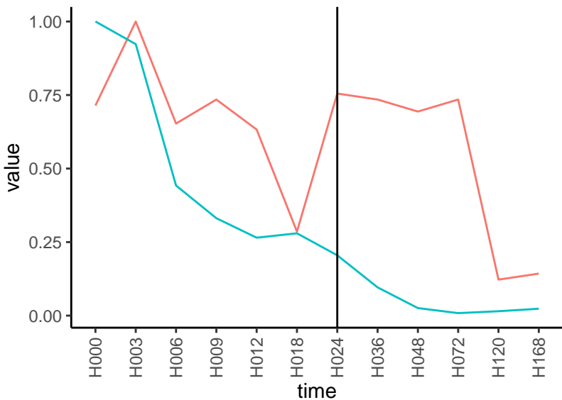
Normalized signals – ENSG00000133067 pre-not-downregulated/post-not-downregula
