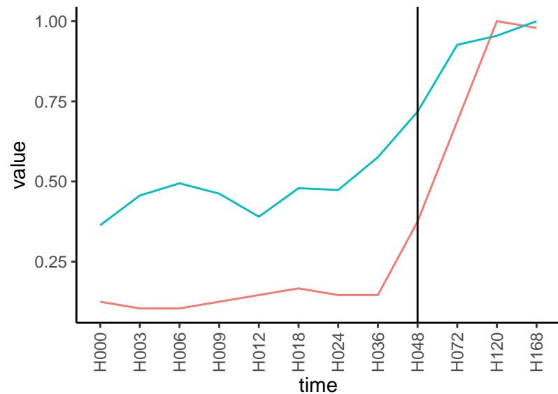
Normalized signals – ENSG00000123643 pre-not-upregulated/post-not-upregulated
