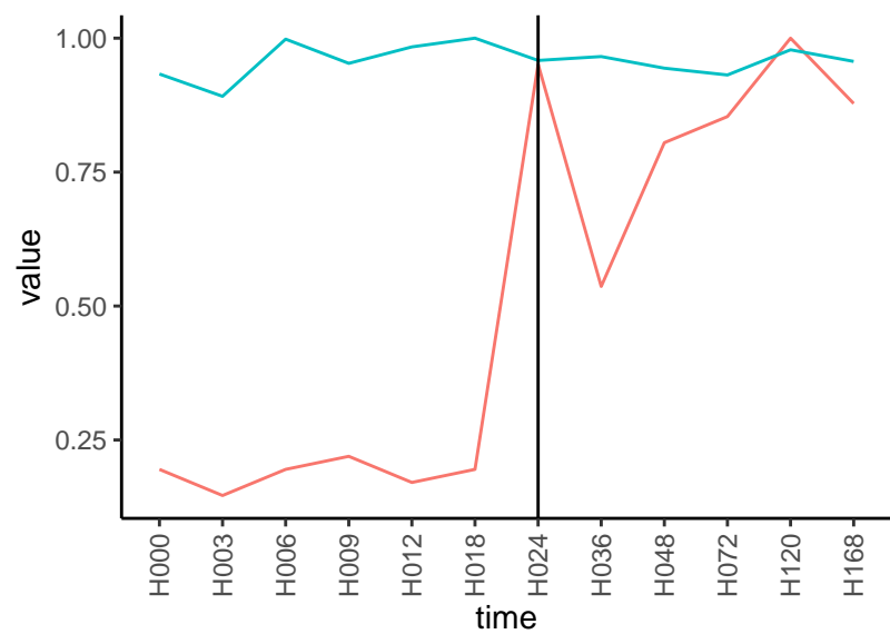
Normalized signals – ENSG00000104957 pre-not-upregulated/post-not-upregulated
