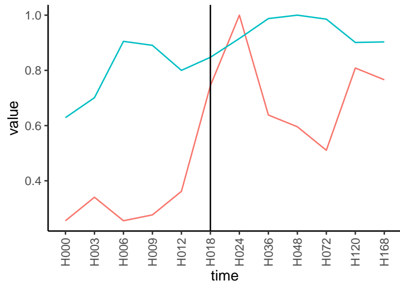
Normalized signals – ENSG00000091490 pre-not-upregulated/post-not-upregulated
