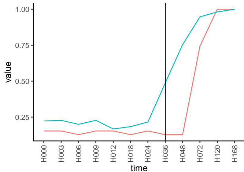
Normalized signals – ENSG00000138640 pre-not-upregulated/post-upregulated
