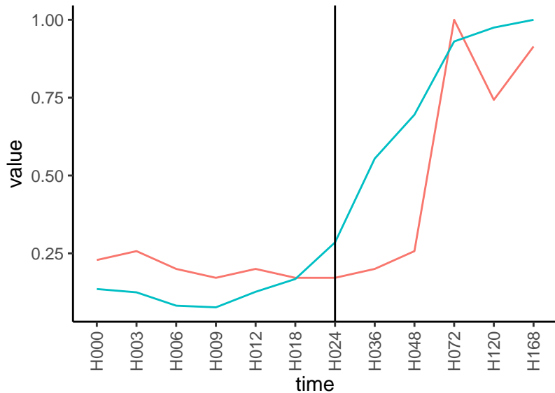
Normalized signals – ENSG00000167851 pre-not-upregulated/post-upregulated
