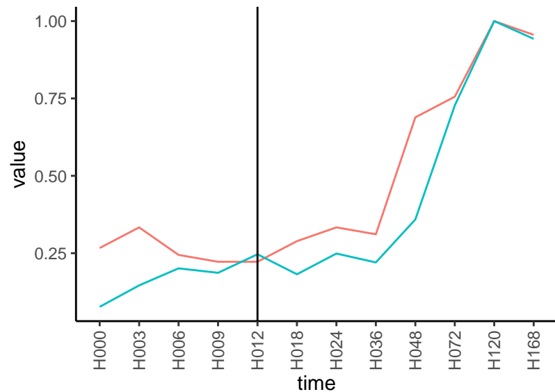
Normalized signals – ENSG00000178726 pre-not-upregulated/post-upregulated
