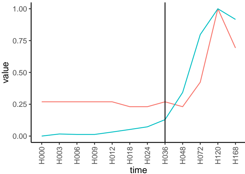
Normalized signals – ENSG00000019169 pre-not-upregulated/post-upregulated
