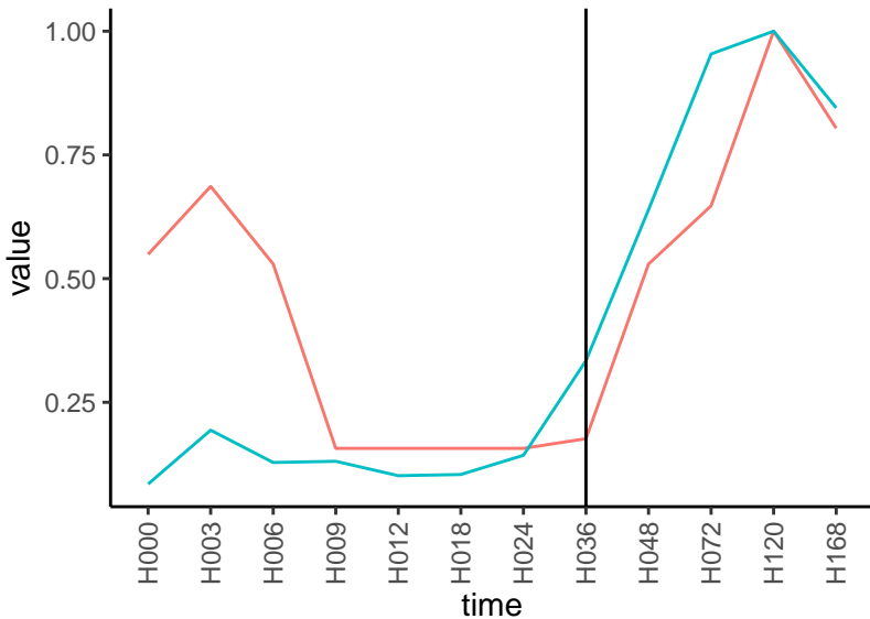
Normalized signals – ENSG00000173166 pre-not-upregulated/post-upregulated
