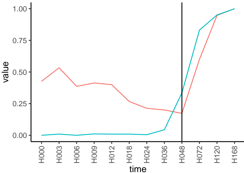
Normalized signals – ENSG00000174600 pre-not-upregulated/post-upregulated
