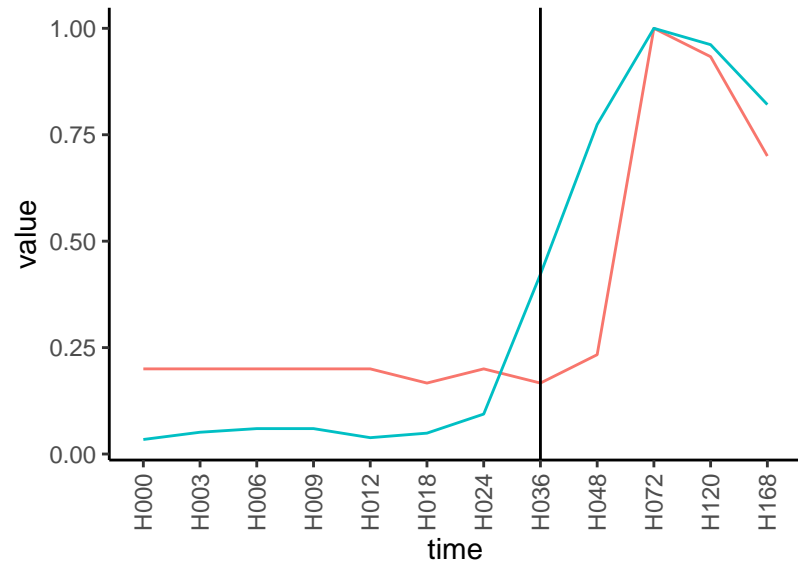
Normalized signals – ENSG00000152315 pre-not-upregulated/post-upregulated
