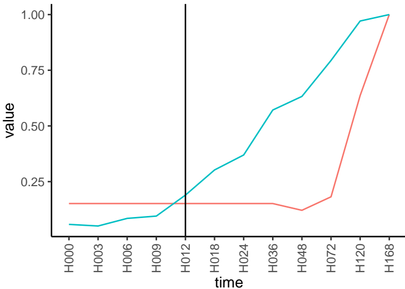
Normalized signals – ENSG00000110077 pre-not-upregulated/post-upregulated
