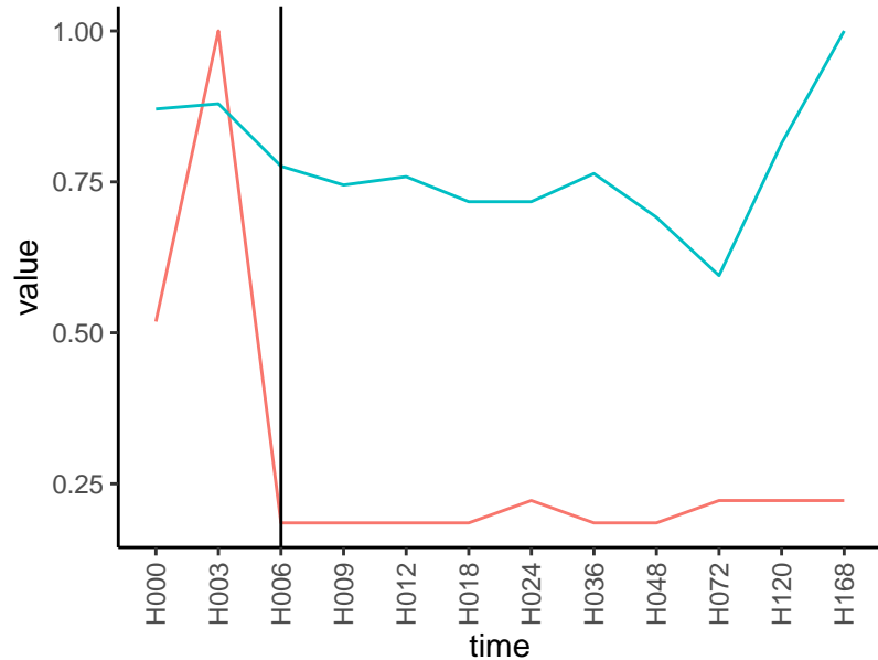
Normalized signals – ENSG00000118292
