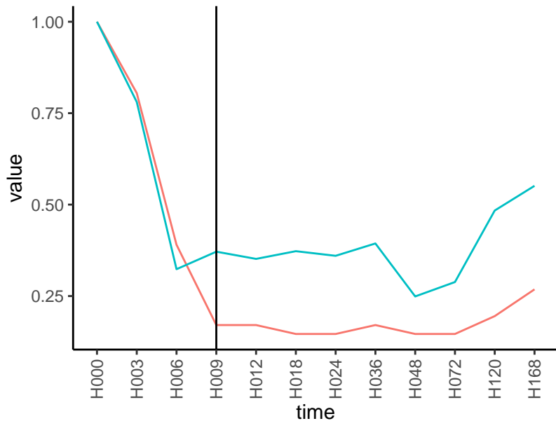
Normalized signals – ENSG00000095585
