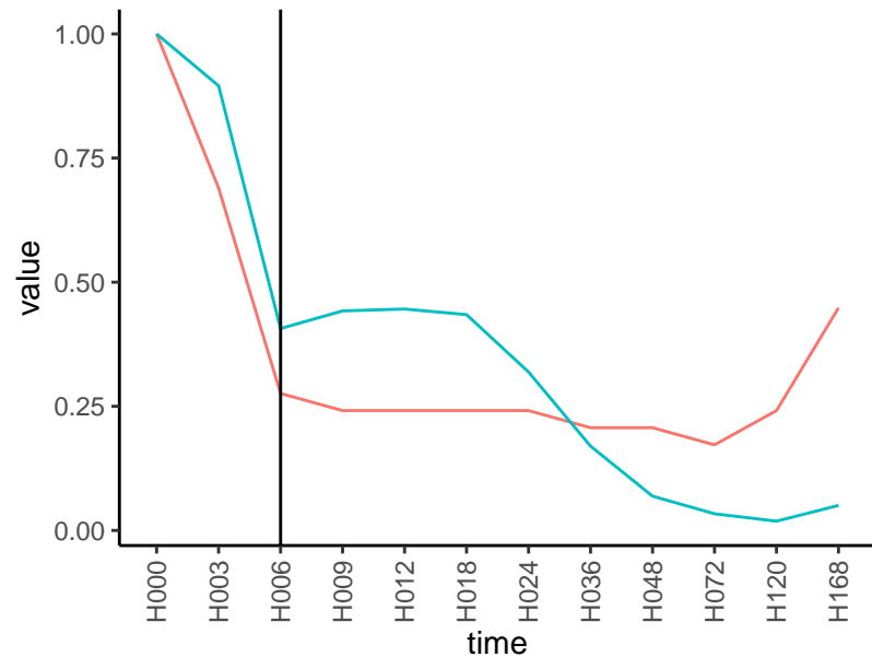
Normalized signals – ENSG00000172995
