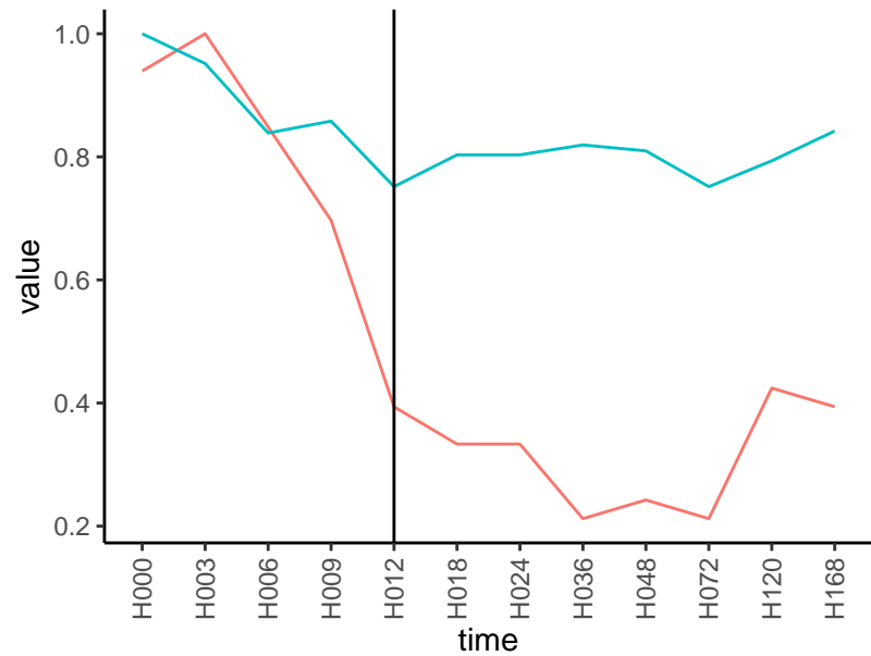
Normalized signals – ENSG00000178917
