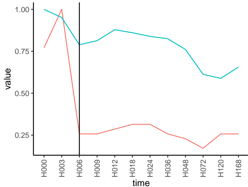
Normalized signals – ENSG00000136104
