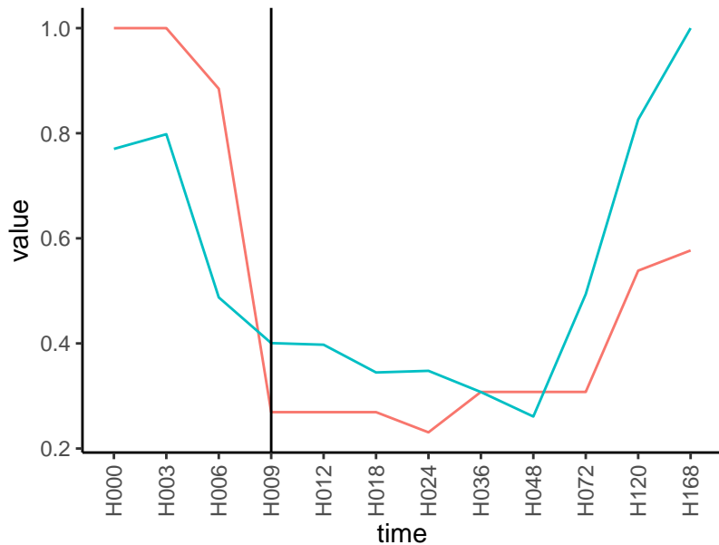
Normalized signals – ENSG00000165959
