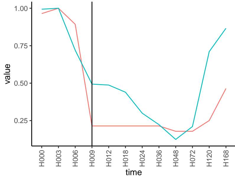
Normalized signals – ENSG00000107518
