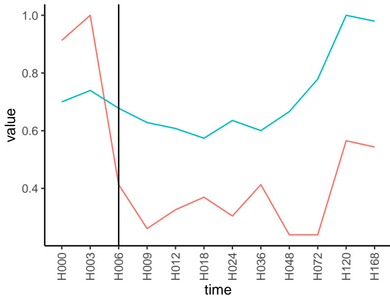
Normalized signals – ENSG00000187837
