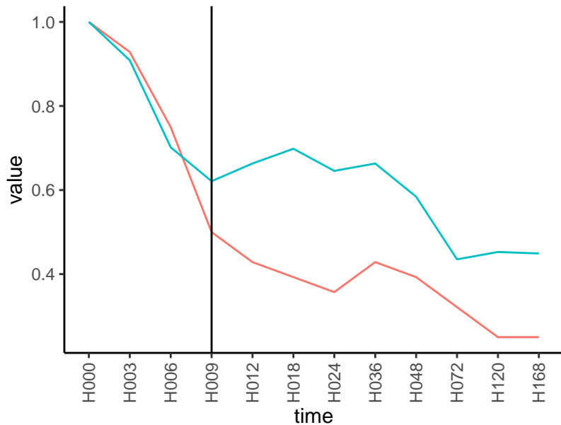
Normalized signals – ENSG00000117480
