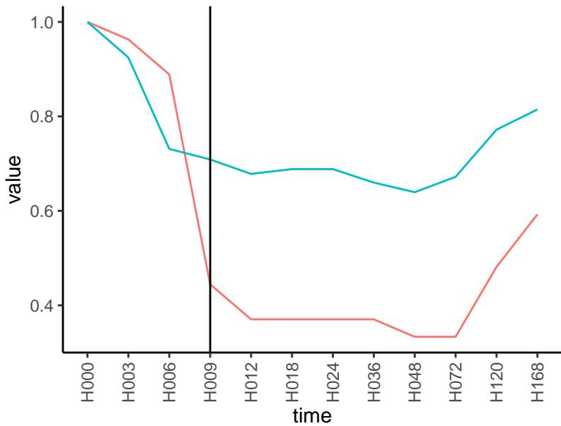
Normalized signals – ENSG00000162139
