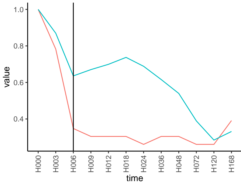
Normalized signals – ENSG00000112294
