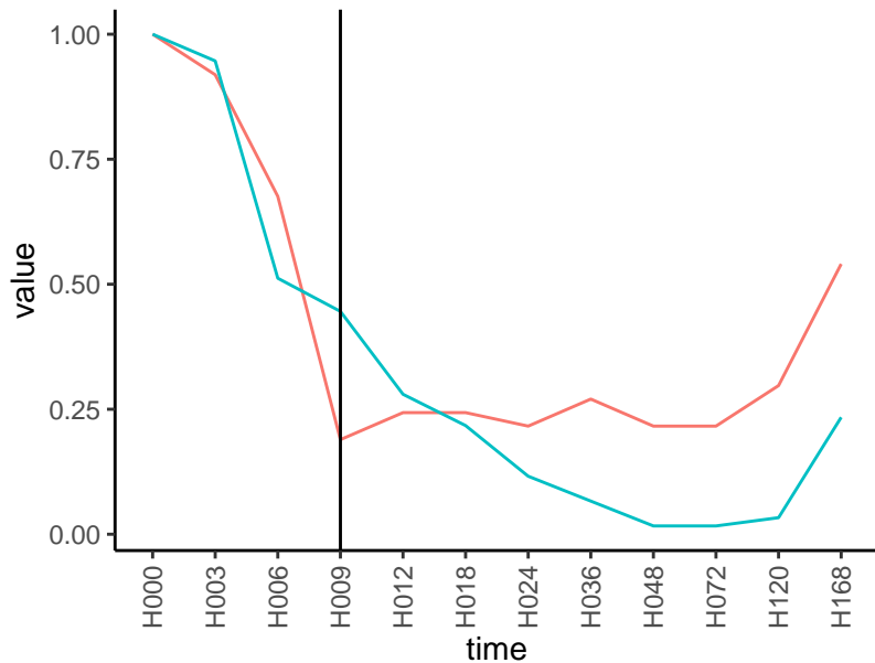
Normalized signals – ENSG00000183117
