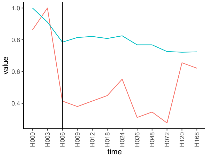
Normalized signals – ENSG00000263465
