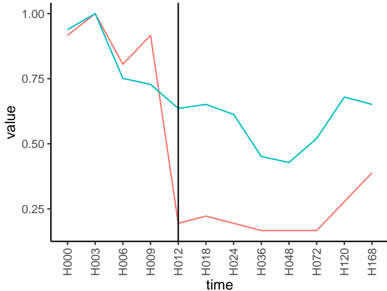
Normalized signals – ENSG00000152894
