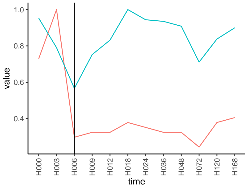
Normalized signals – ENSG00000010318
