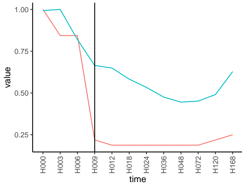
Normalized signals – ENSG00000027075
