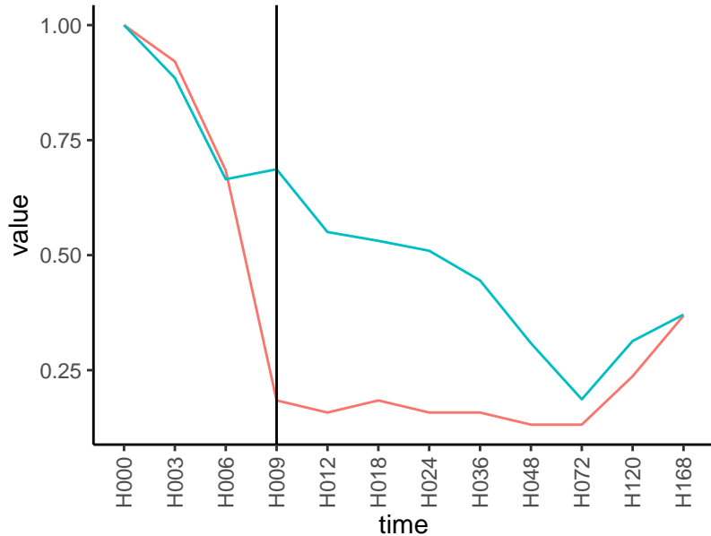
Normalized signals – ENSG00000106415
