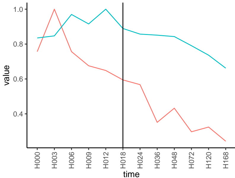
Normalized signals – ENSG00000174109
