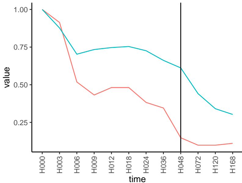
Normalized signals – ENSG00000272398
