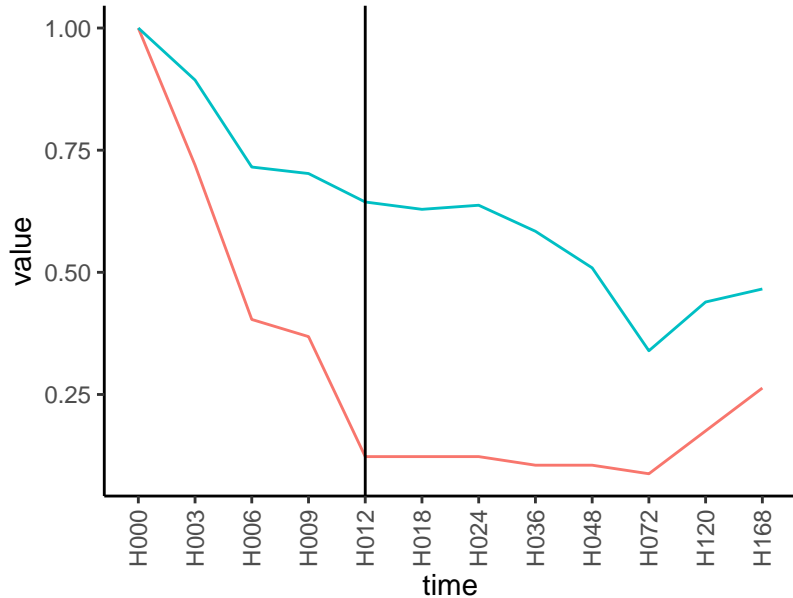
Normalized signals – ENSG00000139737
