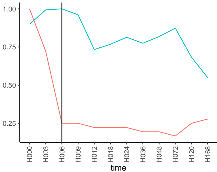
Normalized signals – ENSG00000067715
