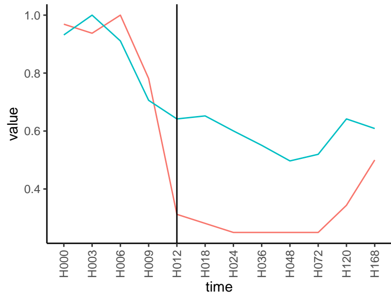
Normalized signals – ENSG00000154153
