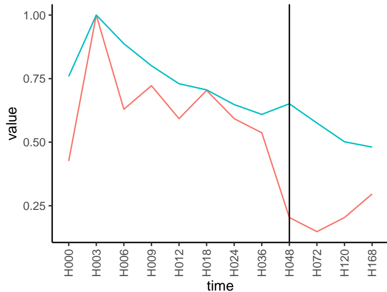
Normalized signals – ENSG00000154640
