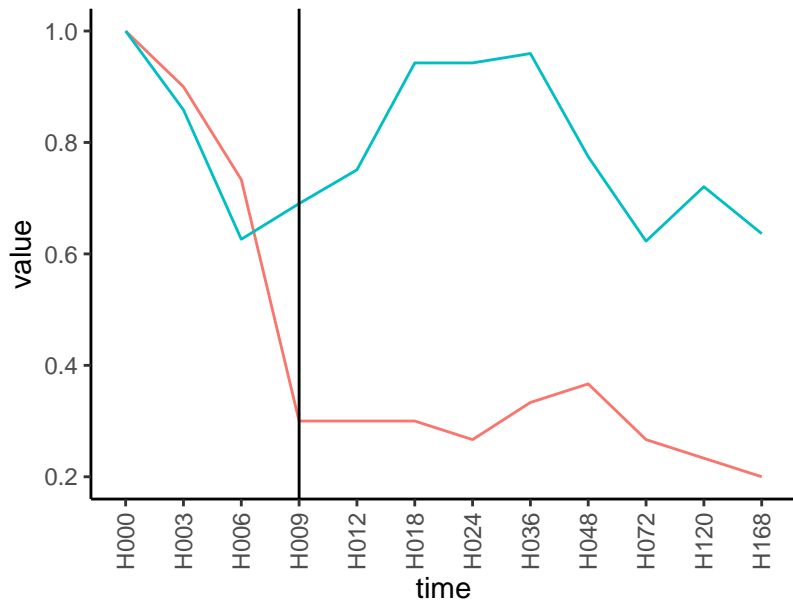
Normalized signals – ENSG00000110237
