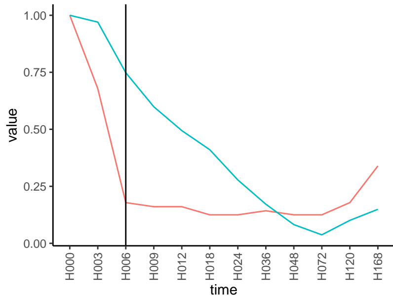
Normalized signals – ENSG00000165078
