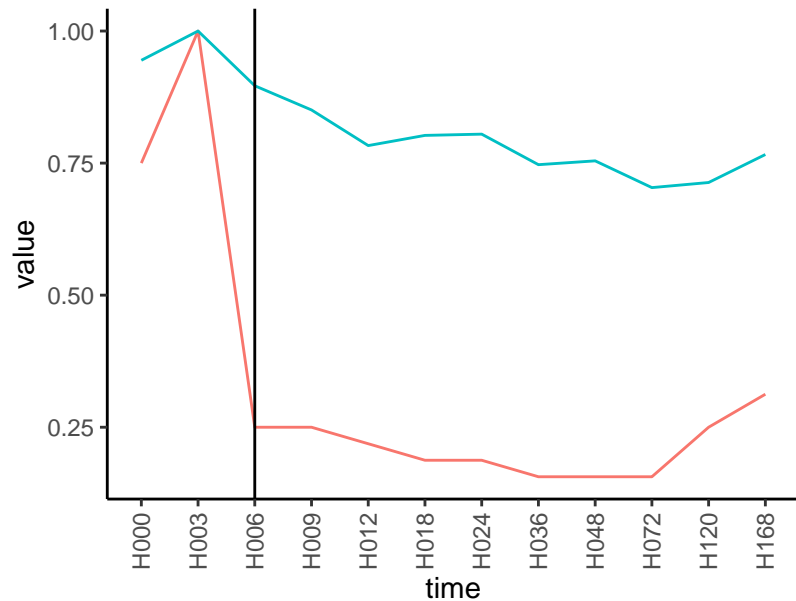
Normalized signals – ENSG00000186020
