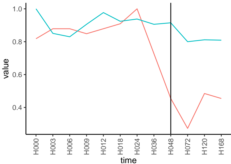
Normalized signals – ENSG00000171103 pre-not-downregulated/post-not-downregulat
