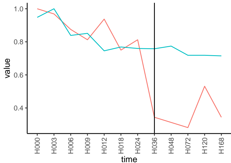
Normalized signals – ENSG00000197961 pre-not-downregulated/post-not-downregulat
