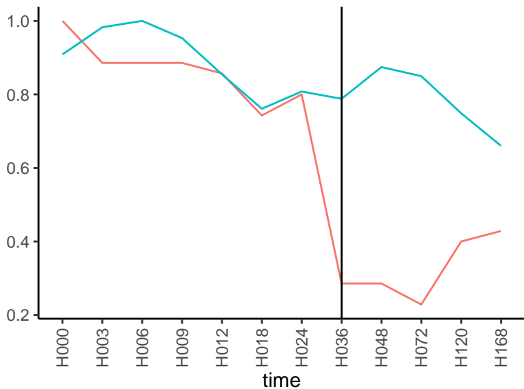
Normalized signals – ENSG00000156017 pre-not-downregulated/post-not-downregulat
