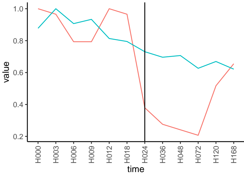
Normalized signals – ENSG00000196911 pre-not-downregulated/post-not-downregulat
