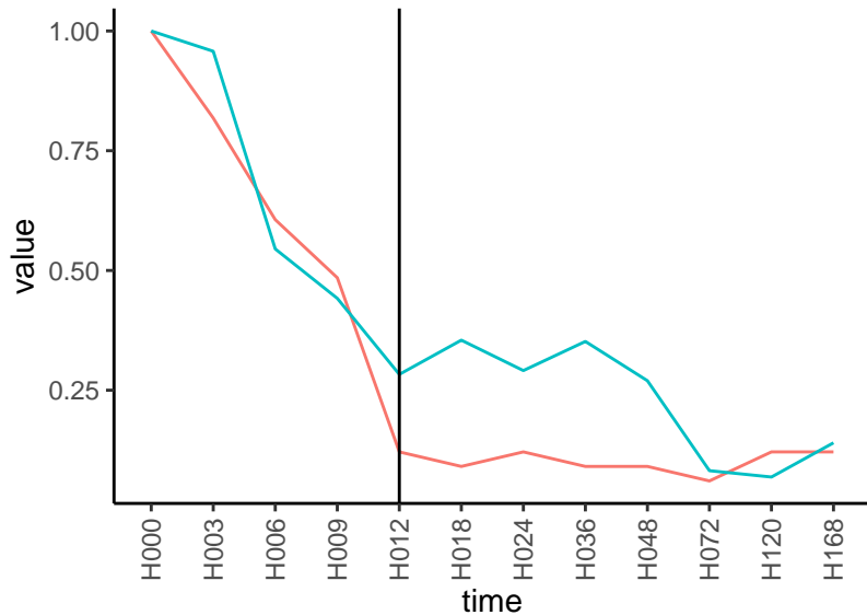
Normalized signals – ENSG00000112182 pre-not-downregulated/post-downregulated
