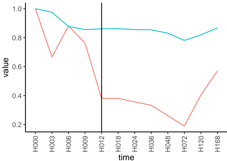
Normalized signals – ENSG00000104231 pre-not-downregulated/post-not-downregulat
