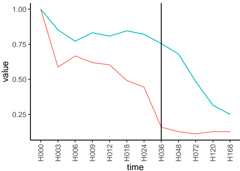
Normalized signals – ENSG00000118513 pre-not-downregulated/post-not-downregula
