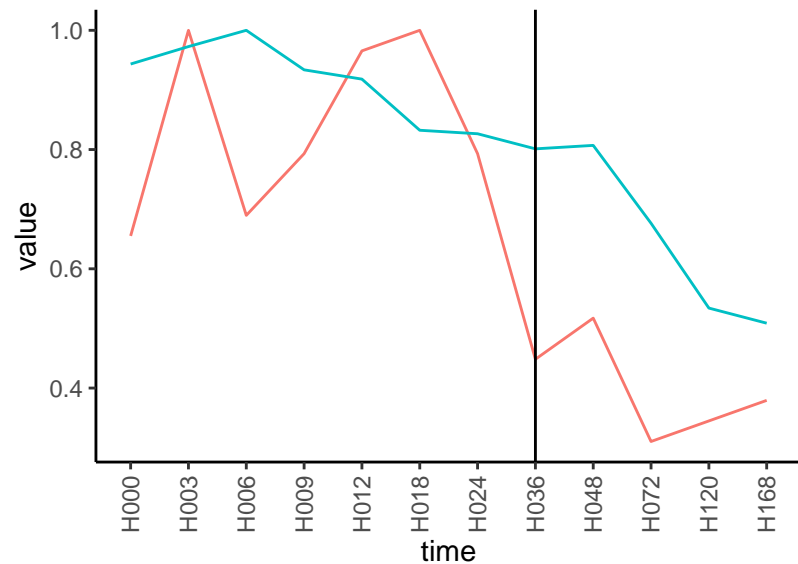
Normalized signals – ENSG00000126953 pre-not-downregulated/post-downregulated
