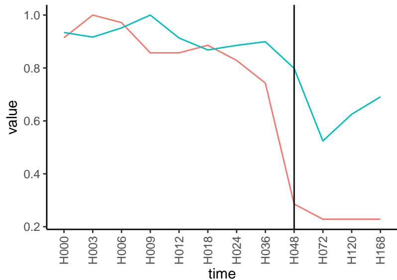
Normalized signals – ENSG00000184083 pre-not-downregulated/post-not-downregulat
