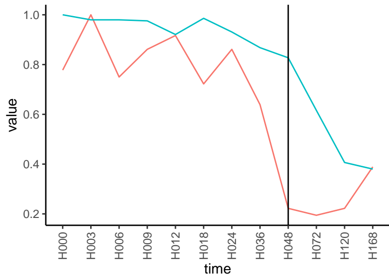
Normalized signals – ENSG00000152990 pre-not-downregulated/post-not-downregulat
