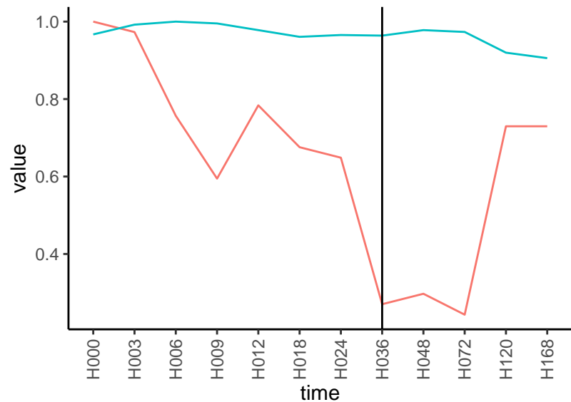
Normalized signals – ENSG00000171566 pre-not-downregulated/post-not-downregulat
