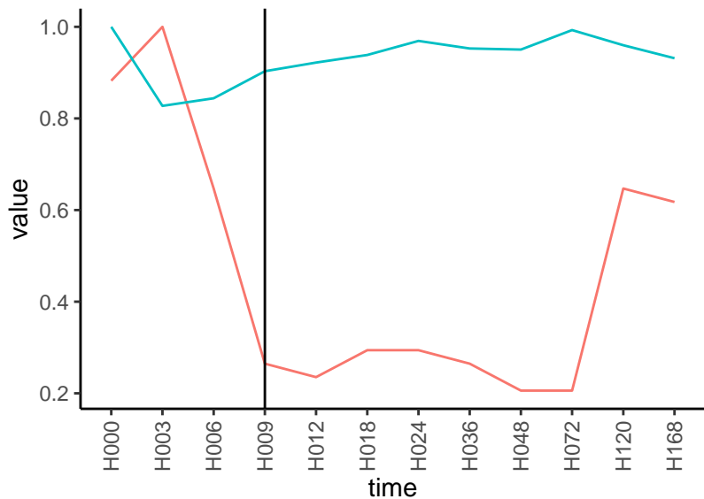
Normalized signals – ENSG00000164252 pre-not-downregulated/post-not-downregulat
