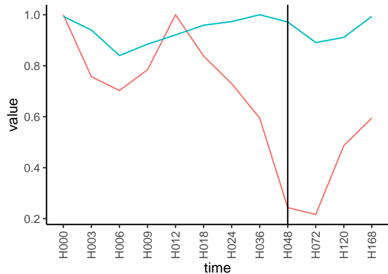
Normalized signals – ENSG00000121691 pre-not-downregulated/post-not-downregulat
