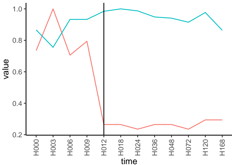
Normalized signals – ENSG00000063176 pre-not-downregulated/post-not-downregulat
