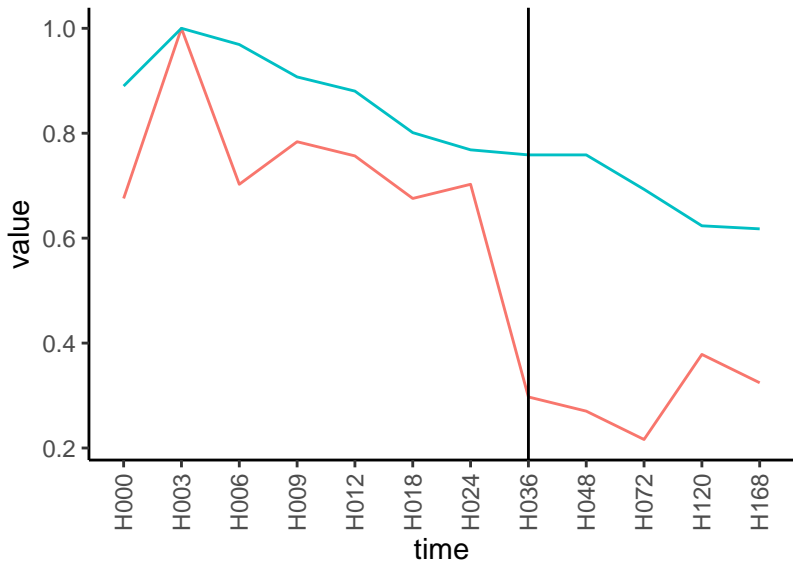
Normalized signals – ENSG00000133641 pre-not-downregulated/post-not-downregulat
