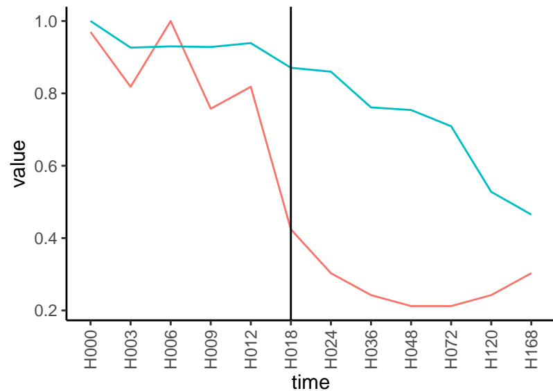
Normalized signals – ENSG00000158234 pre-not-downregulated/post-downregulated
