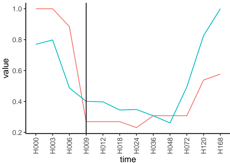
Normalized signals – ENSG00000165959 pre-not-downregulated/post-not-downregulat
