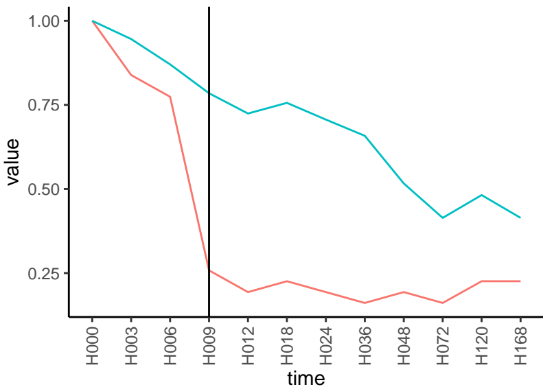
Normalized signals – ENSG00000004468 pre-not-downregulated/post-not-downregula
