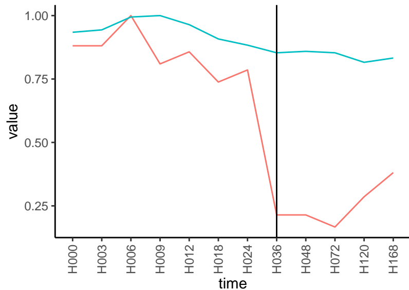
Normalized signals – ENSG00000005175 pre-not-downregulated/post-not-downregula
