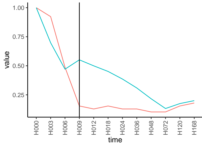
Normalized signals – ENSG00000166349 pre-not-downregulated/post-downregulated
