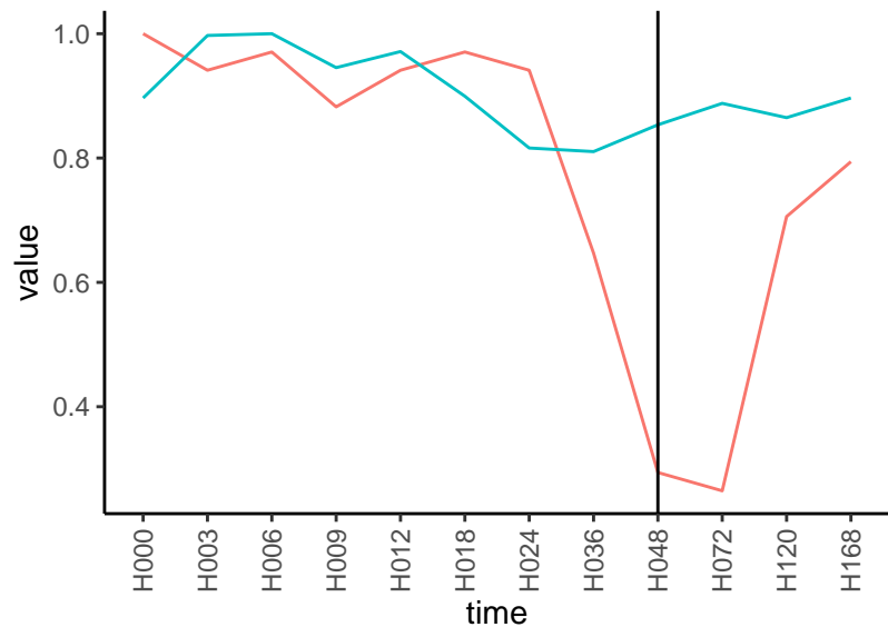
Normalized signals – ENSG00000116095 pre-not-downregulated/post-not-downregulat
